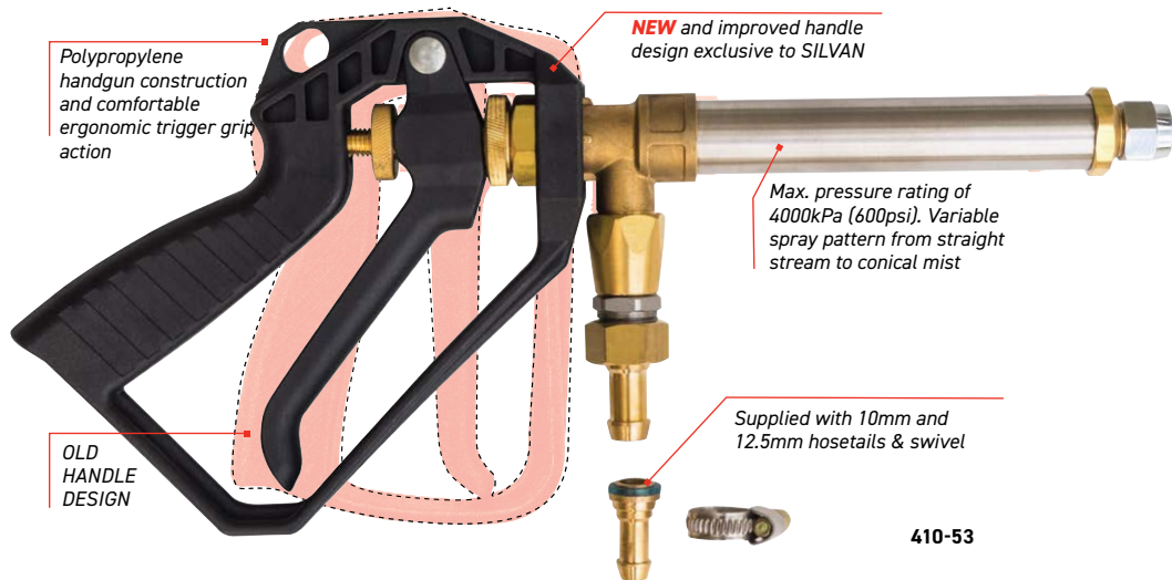
PENCIL STREAM IS IDEAL FOR HERBICIDE AND DISTANCE SPRAYING
